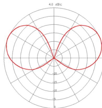
ELEVATION PATTERN
